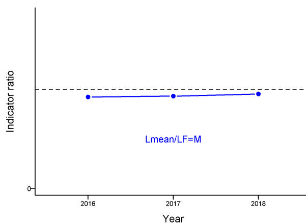
Figure 2 Horse mackerel in divisions 3.a, 4.b–c, and 7.d. The index ratio L_{\text{mean}}/L_{F=M} from the length-based indicator (LBI; ICES, 2018a) method is used for the evaluation of the exploitation status. The exploitation status is above the F_{\text{MSY}} proxy when the index ratio value is less than 1, which is indicated by the dashed line.
